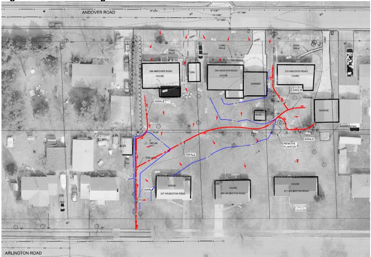
Figure 1 – Yard Grading.
